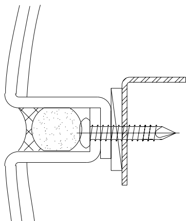
7. VERTICAL JOINT
