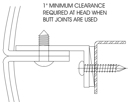
8. ALTERNATE BUTT JOINT
