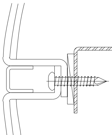
7A. ALTERNATE JOINT
