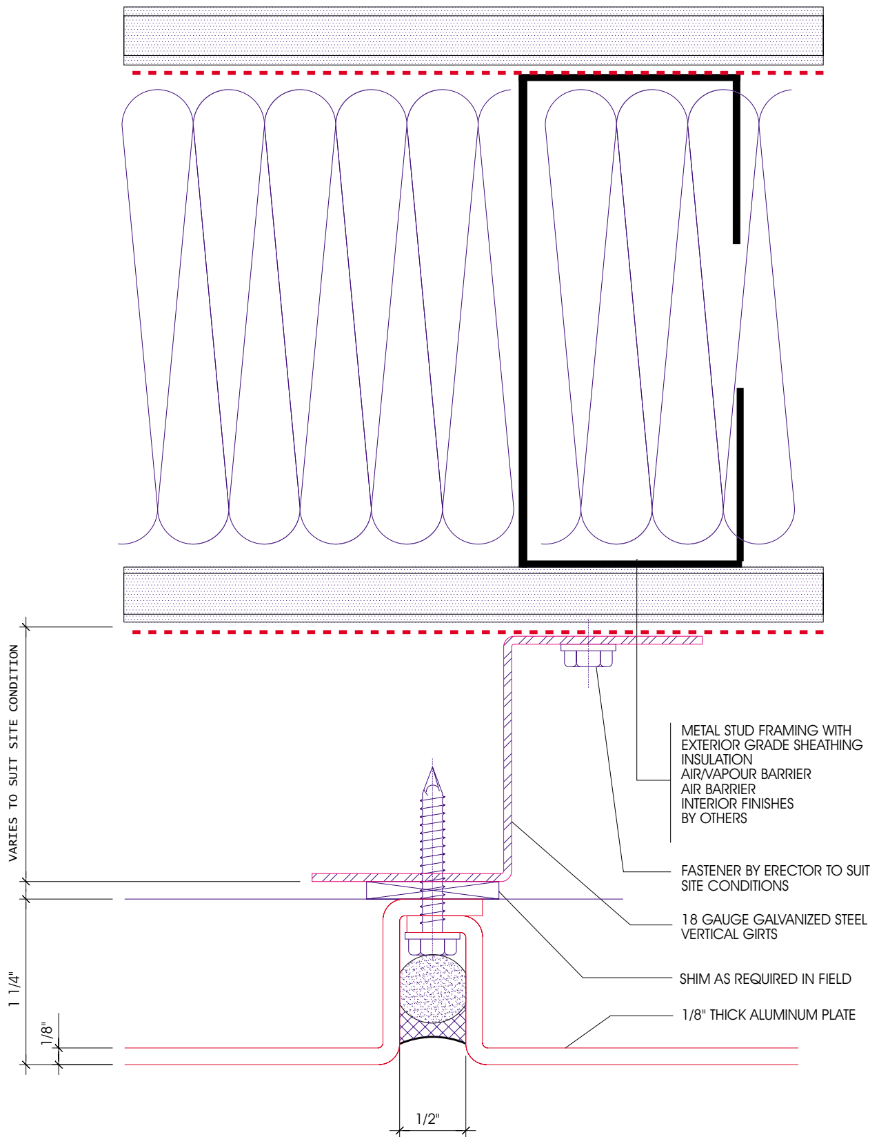
4. VERTICAL JOINT
